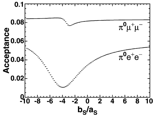
Fig. 6. Overall acceptance as a function of b_S/a_S for the K_S \rightarrow \pi^0 \mu^+ \mu^- (upper curve) and K_S \rightarrow \pi^0 e^+ e^- (lower curve) channels.
