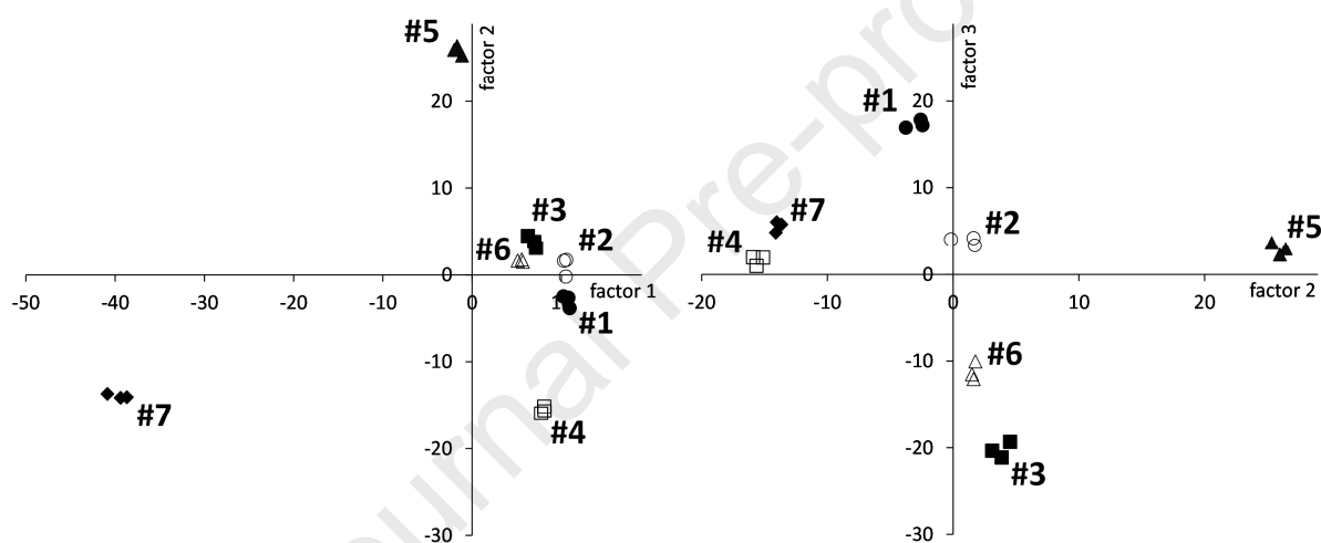
Figure 4. Mode 1 loadings plots of PARAFAC model (factor 1 vs. 2 and factor 2 vs. 3) representing effect of the material type on the natural weathering extent.
