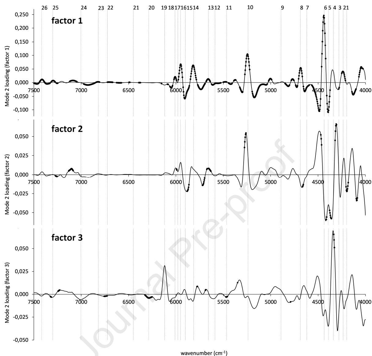
Figure 7. Mode 2 loadings revealing a contribution of the near infrared spectrum on the PARAFAC model describing biomaterials deterioration kinetics. Note: Spectral range reduced to 4000 - 7500\text{cm}^{-1} , the highlighted points correspond to variables that have congruence loadings >0.6 .
