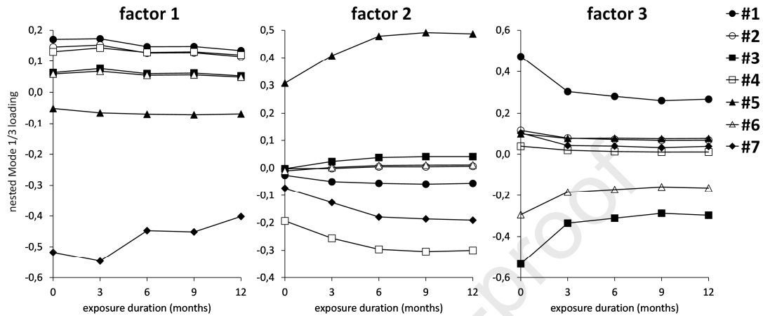
Figure 5. Nested loadings Mode 1/3 biplot for the three factors of PARAFAC model for the natural weathering of modified wood.
