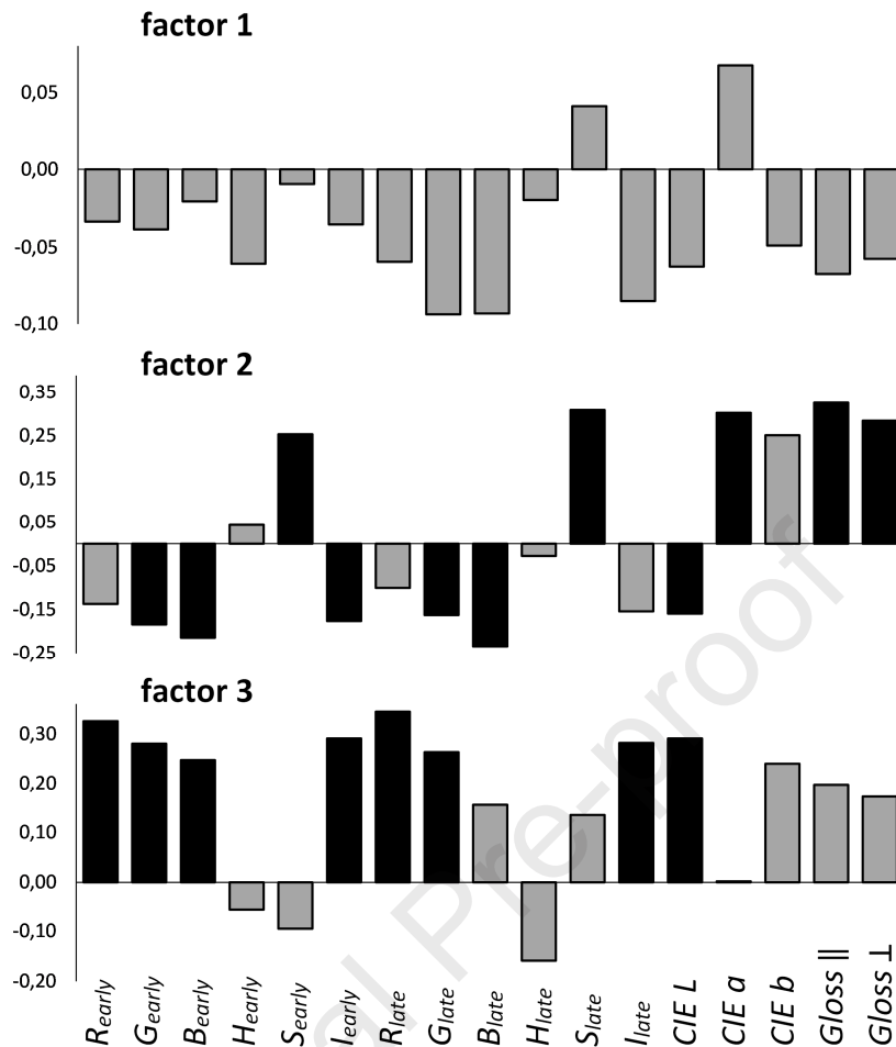
Figure 8. Mode 2 loadings revealing a contribution of the surface appearance (colour and gloss) on the PARAFAC model describing biomaterials deterioration kinetics. The highlighted variables have congruence loadings >0.6.
