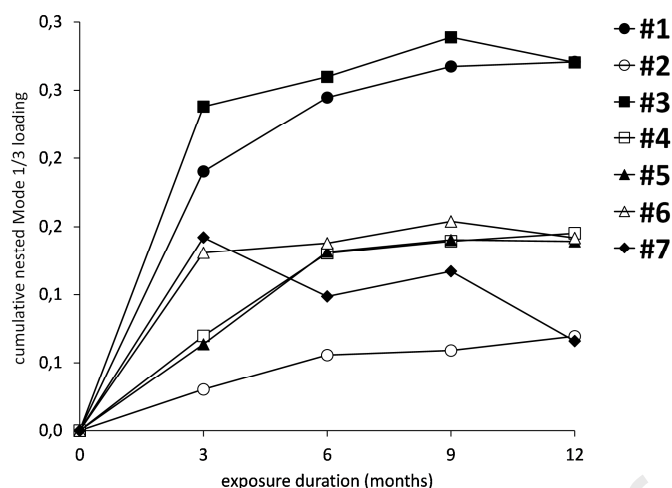
Figure 6. Cumulative nested biplot for Mode 1/3 loadings of PARAFAC model for seven modified wood samples exposed to natural weathering.
