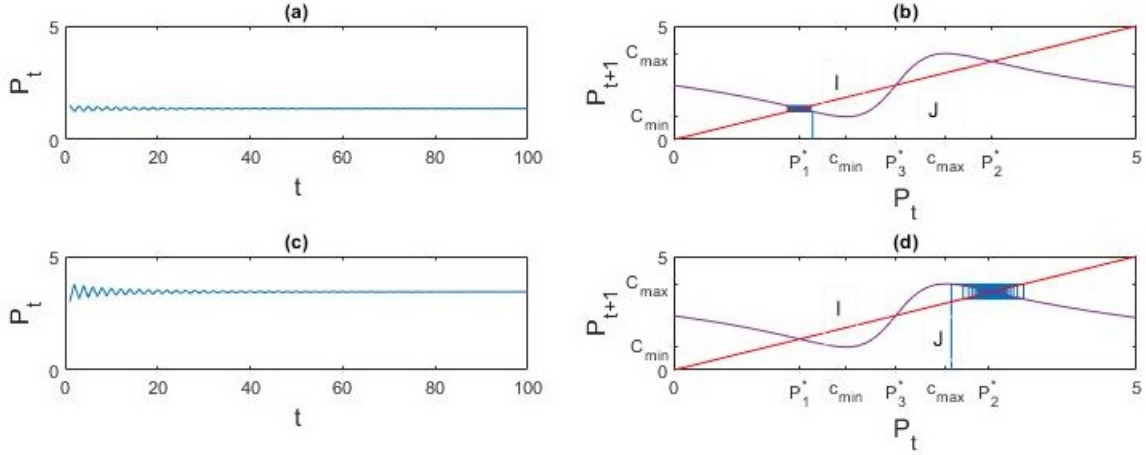
Figure 2: Coexistence of attractors for parameters n_2 = 0.5 , F_1 = 3.44 , F_2 = 1.36 , \lambda = 1.3 , N = 0.5 . In (a) and (b) (greed scenario) an i.c. P_0 = 1.5 generates a trajectory converging to the fixed point P_1^* . While in (c) and (d) (fear scenario), for P_0 = 3 the trajectory converges to the fixed point P_2^* .
