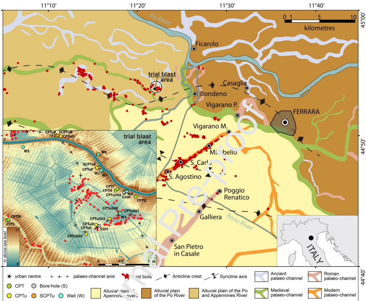
Fig. 1. Map of the palaeo-channel bodies (modified after Stefani et al., 2018), of the surface manifestations of liquefaction following the 2012 Emilia-Romagna earthquake (Emergeo Working Group, 2013) and of the location of the blast area. The traces of the main anticline crest and syncline axis of the buried tectonic belt are also depicted. The lower-left corner shows the geomorphological features from LIDAR map together with the available investigations and the 2012 sand boils.
