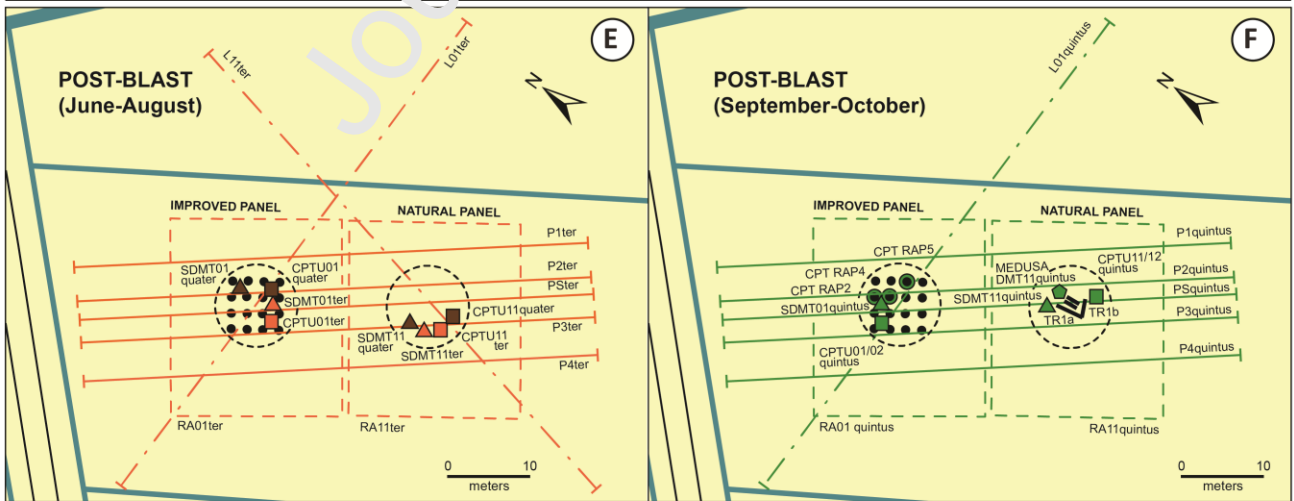
ERT (June-Sept/Oct) Seismic array (June-Sept/Oct) ●●● CPT RAP Trenches (TR) ●●● RAP columns ▲ ▲ ▲ SDMT (June-July/Aug-Sept/Oct) MASW (June-Sept/Oct) Drainage channel ● Blast panel ◆ Medusa DMT (Sept/Oct) ■ ■ ■ CPTU (June-July/Aug-Sept/Oct)
