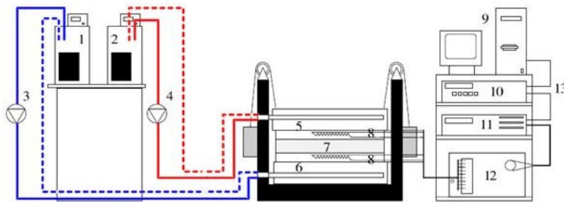
Figure 1 - Illustrative chart and general view of Bologna heat flow meter apparatus. 1), 2) thermostatic baths; 3), 4) circulator pumps; 5), 6) heating and cooling plates; 7) test specimen; 8) heat flow meters; 9) personal computer; 10) multimeter; 11) switcher unit; 12) ice point; 13) general purpose interface bus.
