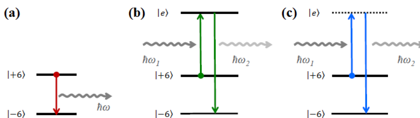
Figure 8. Spin-lattice relaxation processes. (a) Direct relaxation into the ground state involving the emission of a phonon with energy \hbar\omega . (b) Two-phonon Orbach process, in which the molecule is excited into the state |e\rangle via the absorption of a phonon of energy \hbar\omega_1 and subsequently emits another phonon of energy \hbar\omega_2 , thereby relaxing into its ground state. (c) Two-phonon Raman process, similar to the Orbach one but involving a virtual excited state. Hyperfine splitting of the ground state doublet was omitted for simplicity.
