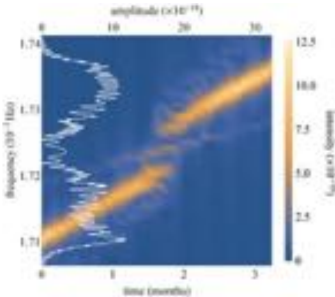
Fig. 34 Periodogram of the fundamental frequency of a gravitational waveform associated with an inspiral on a particular non-Kerr spacetime. A sudden jump in the frequency evolution appears when the inspiralling object crosses a Birkhoff island, which is associated with a valley in the amplitude of the signal's frequencies (white line)
