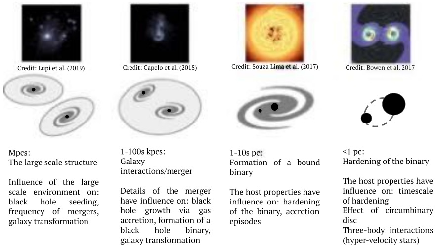
Fig. 16 A schematic view of the complex and multi-scale processes affecting the formation of a hard MBH binary system. Image credit: Silvia Bonoli and Alessandro Lupi
