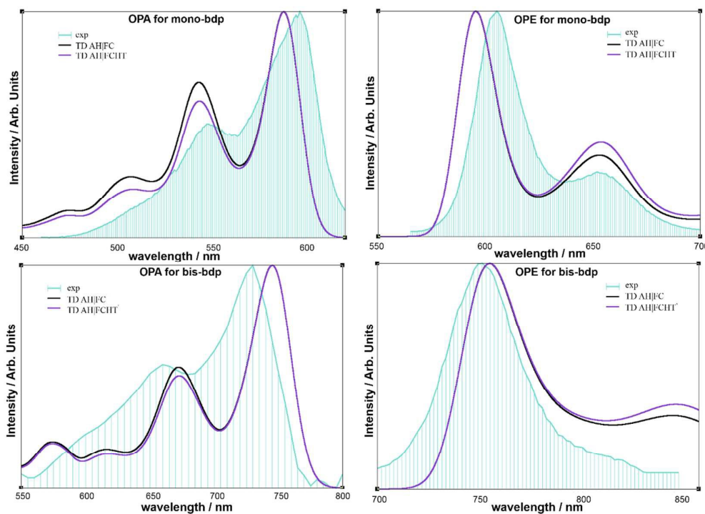
Figure 6. Vibronic absorption and emission spectra of mono-bdp and bis-bdp , computed at the TD AH|FC and TD AH|FC|HT levels, with the MN15 density functional and neglecting temperature effects, along with the experimental one recorded at 77K in methanol. Gaussian distribution functions with \text{HWHM}=250\text{ cm}^{-1} have been used to simulate the broadening.
