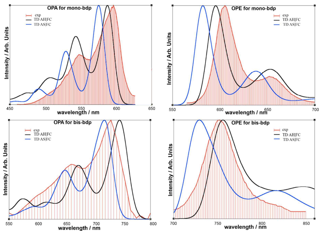
Figure 7. Vibronic absorption and emission spectra of mono-bdp and bis-bdp , computed at the TD AH|FC and TD AS|FC levels, with the MN15 density functional. Gaussian distribution functions with \text{HWHM}=250\text{ cm}^{-1} have been used to simulate the broadening.
