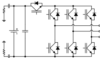
Figure 4. The H7 architecture [14].
