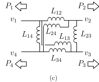
Fig. 4: QAB model. Phase-shift modulation (a), star model (b) and delta model (c).
