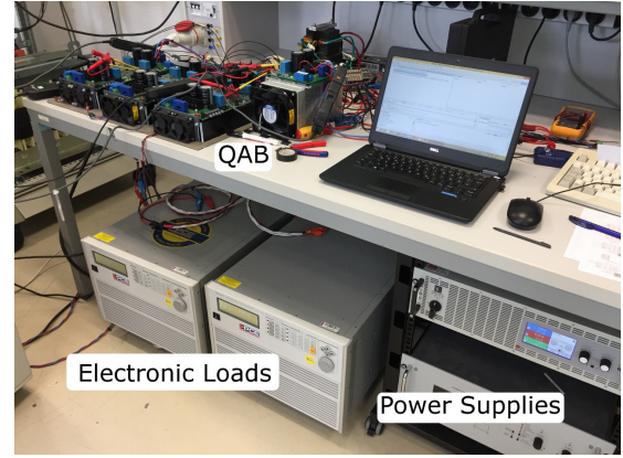
(a) Picture of the experimental setup.
