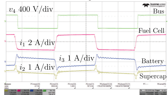
(c) Steady-state.
