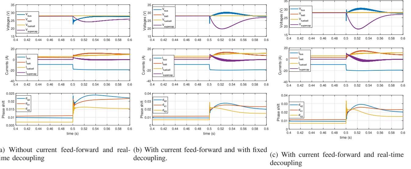
Fig. 11: Simulation results of the QAB with a load step and different control strategies.
