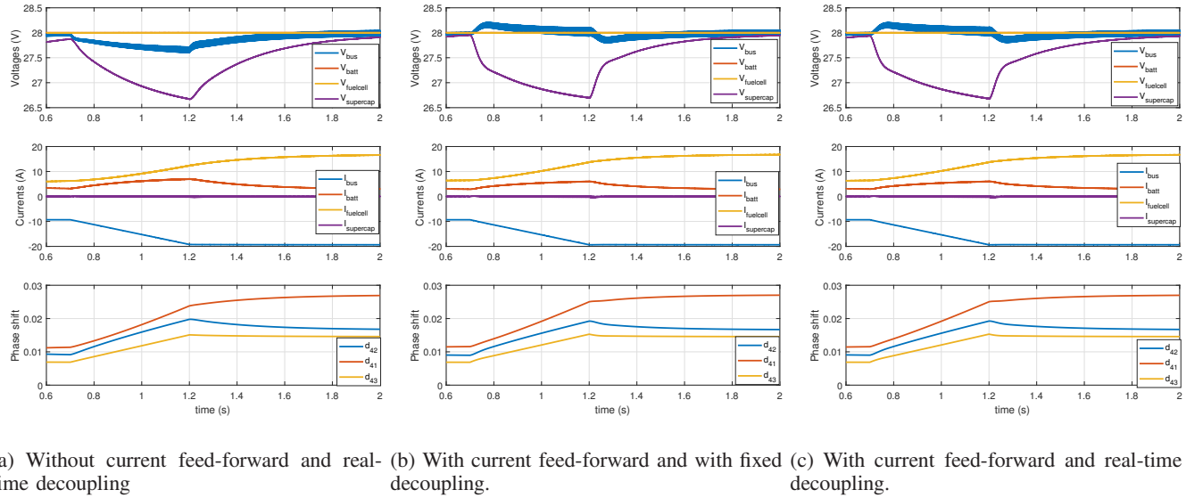
Fig. 12: Simulation results of the QAB in case of a slow load variation.
