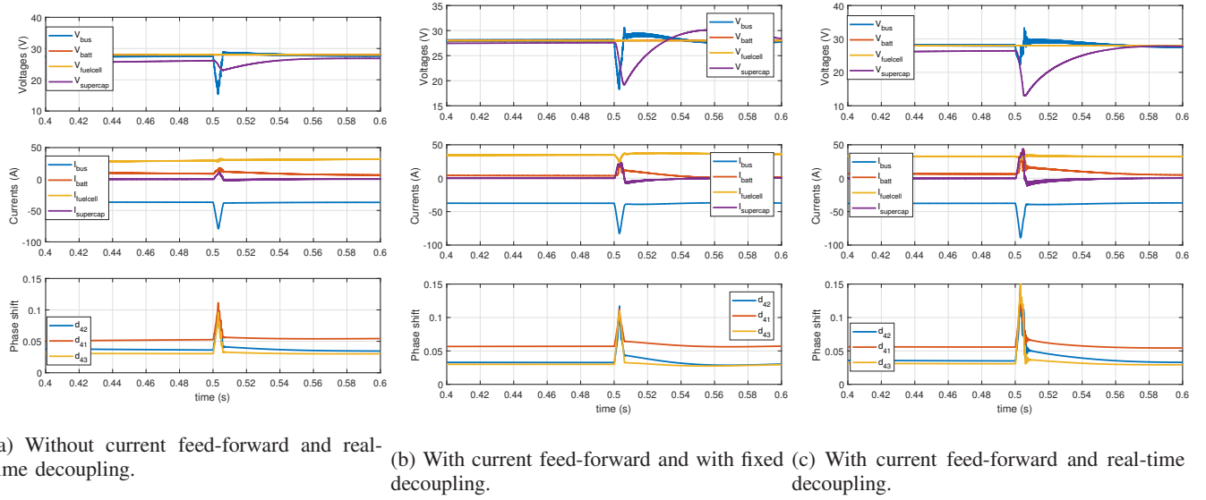
Fig. 13: Simulation results of the QAB during an overload condition, where all three energy sources must supply power.
