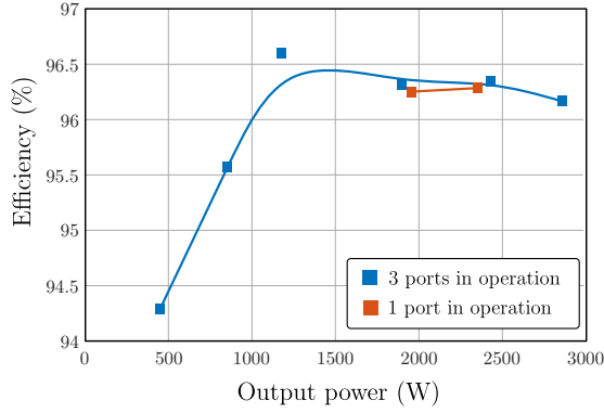
Fig. 16: Efficiency measurement of the QAB converter.
