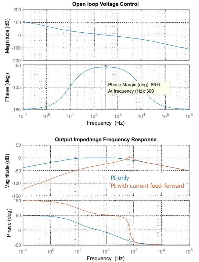
Fig. 8: Frequency response of the voltage control and of the output impedance.
