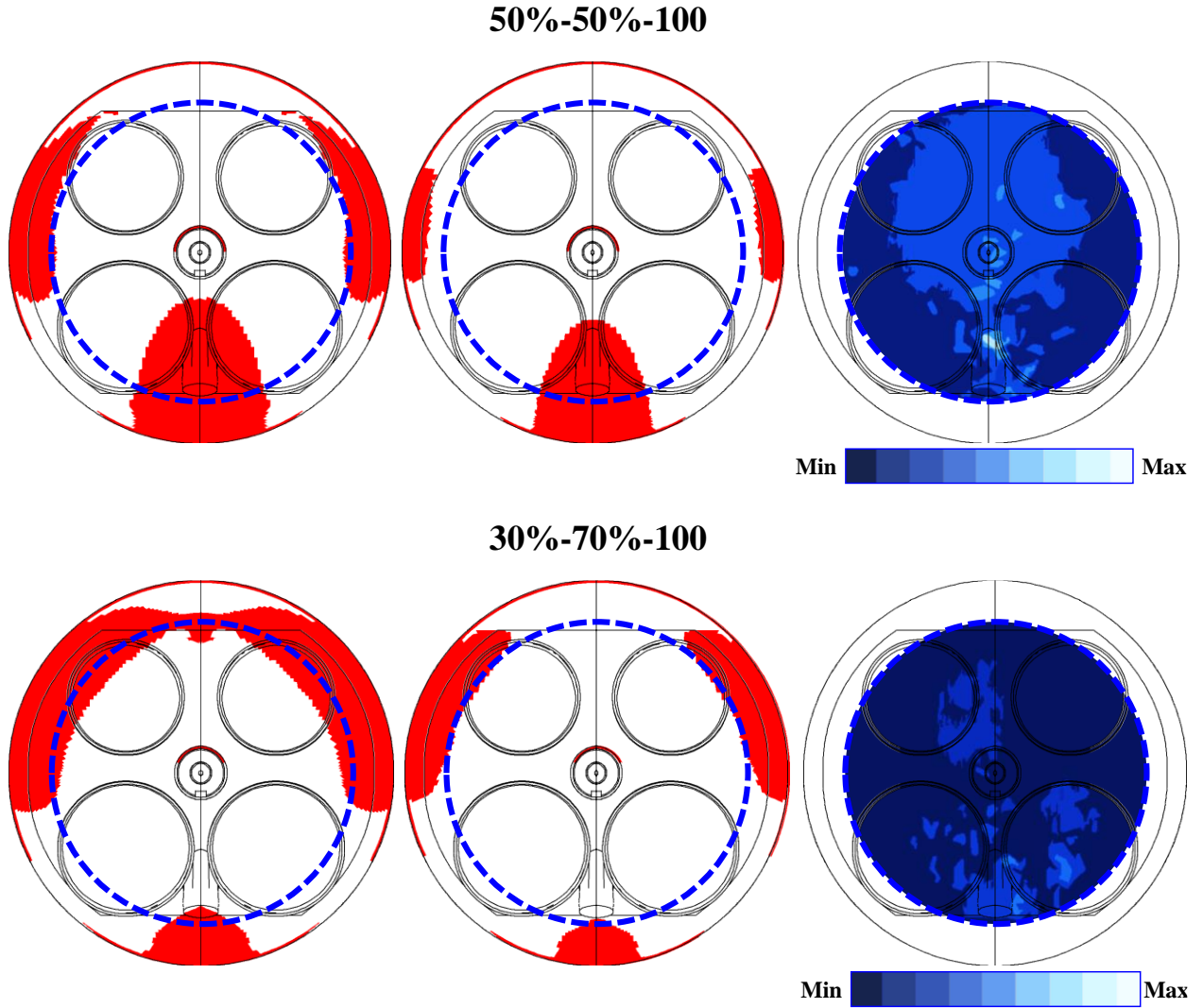
Figure 24: Region with ER > 2 (left) and ER > 2.2 (middle) from numerical simulations at spark timing (30 CAD bTDC) and experimental diffusive flame probability maps (right), for different relative duration of the two injection pulses.
