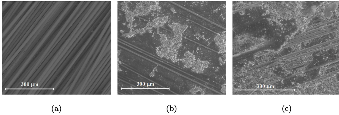
Fig. 9. ESEM micrography at 400\times magnification of G-UC (a) G-ER (b) and G-EW (c) failed specimens.
