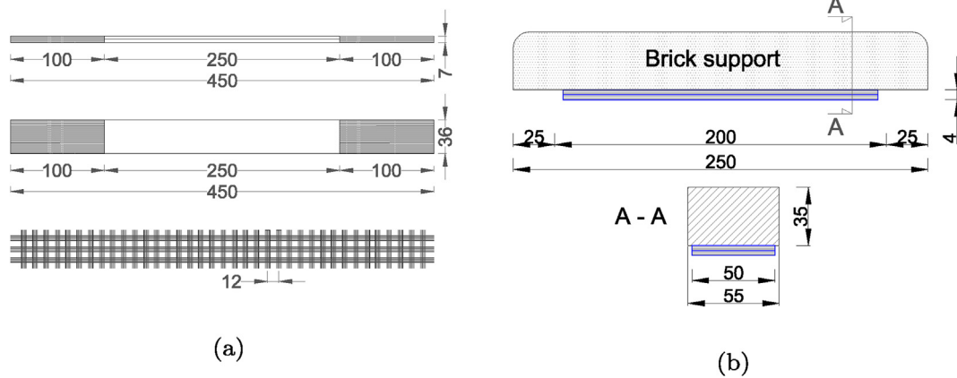
Fig. 2. Specimen geometry (dimensions in mm): (a) rectangular coupons for uni-axial traction test and (b) three-point bending of laminated bricks.
