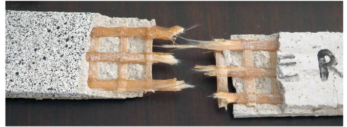
Fig. 6. Fabric rupture is the typical failure mode in the G-ER and G-EW groups under uni-axial traction test.
