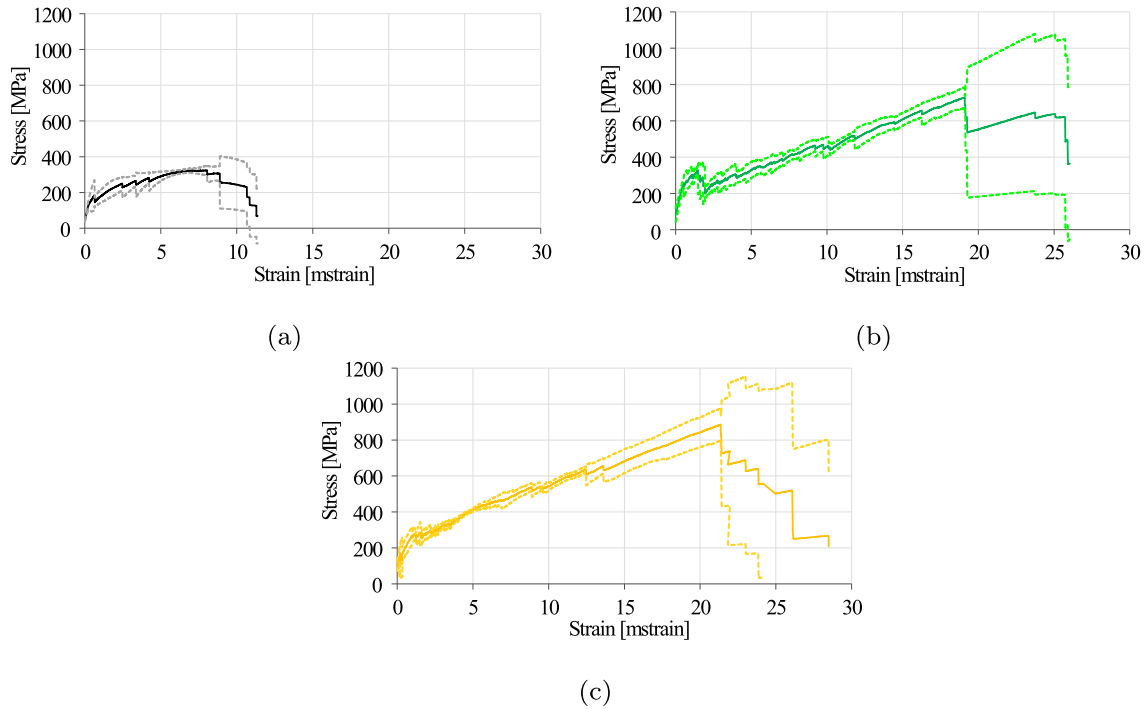
Fig. 12. Mean stress-strain curve with \pm 1 standard deviation band for uni-axial traction of (a) G-UC, (b) G-ER and (c) G-EW specimen groups.
