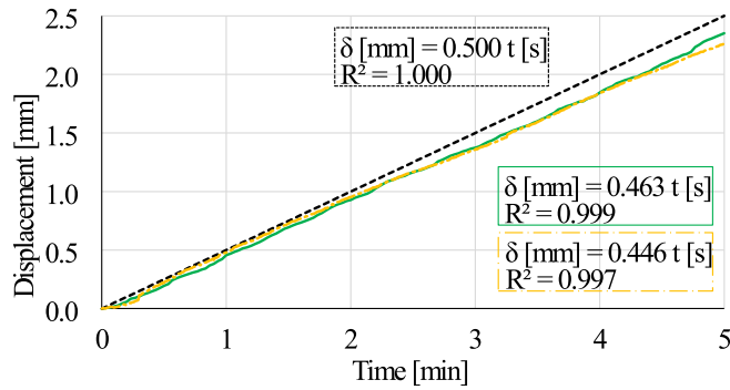
Fig. 4. Uni-axial test nominal elongation ramp imposed at the UTM crosshead (dotted line, black) and actual elongation rate, as measured by DIC, for G-ER (solid, green) and G-EW (dash-dotted, yellow) specimen groups. Linear fitting expressions are also given alongside the coefficient of determination R^2 . (For interpretation of the references to colour in this figure legend, the reader is referred to the Web version of this article.)
