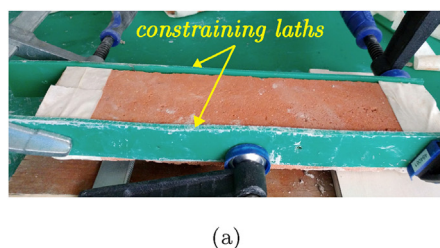
Fig. 3. Three-point bending test specimen manufacture: (a) brick support with constraining laths (b) laminated specimens.
