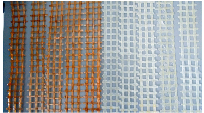
Fig. 1. Coated ARG fabric after cross-linking: G-ER (left) and G-EW (right).
