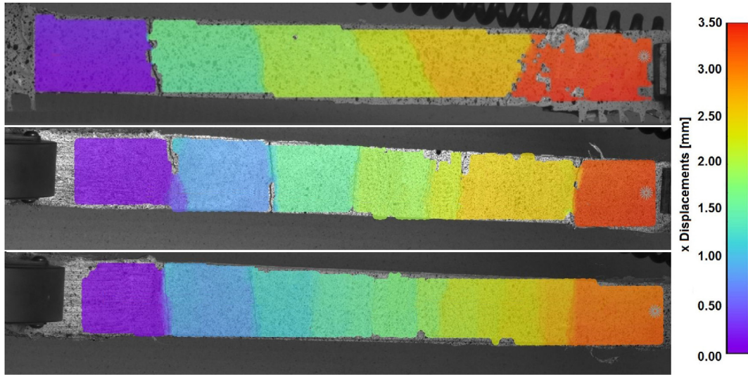
Fig. 14. Longitudinal displacement field for ARG coupons at \varepsilon = 15 mstrain (from top to bottom: G-UC, G-ER and G-EW specimens).
