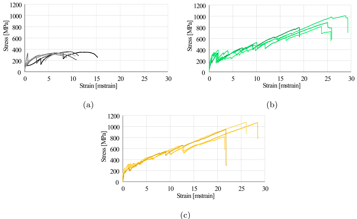
Fig. 11. Stress-strain curves for uni-axial traction of all tested specimens in the G-UC (a) G-ER (b) and G-EW (c) groups.
