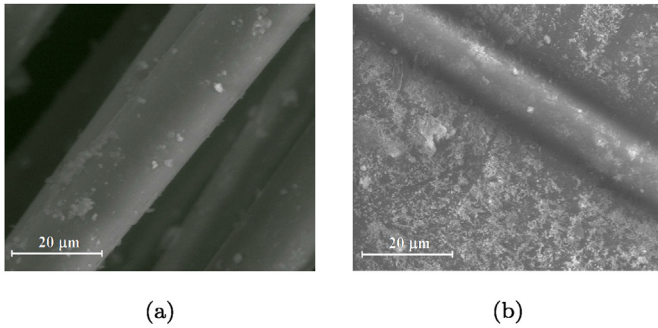
Fig. 10. ESEM micrography at 4000\times magnification of G-UC (a) and G-ER (b) failed specimens.
