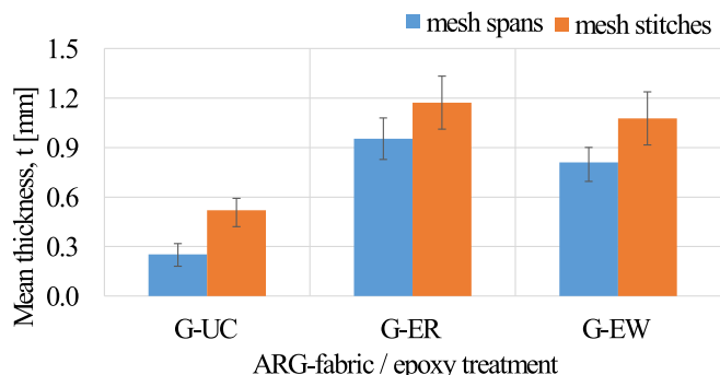
Fig. 5. Mean fabric thickness at the yarns and at the stitches.
