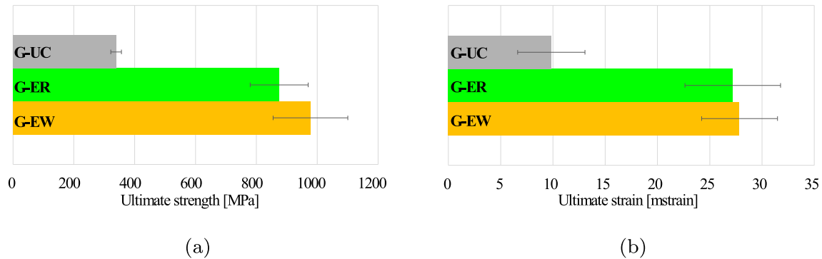
Fig. 13. Mean ultimate stress (a) and mean ultimate strain (b) evaluated in uni-axial traction for all specimen groups.
