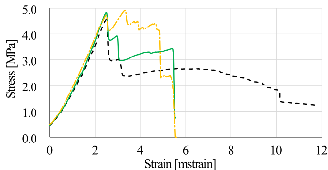
Fig. 17. Mean stress-strain curves for three-point bending of clay bricks laminated with G-UC (dotted, black), G-ER (solid, green) and G-EW (dash-dotted, yellow) composite. (For interpretation of the references to colour in this figure legend, the reader is referred to the Web version of this article.)
