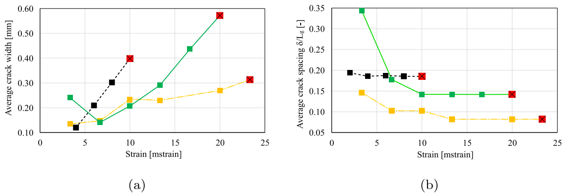
Fig. 16. Mean crack width (a) and dimensionless crack mean spacing (b) vs. strain for G-UC (dotted, black), G-ER (solid, green) and G-EW (dash-dotted, orange). (For interpretation of the references to colour in this figure legend, the reader is referred to the Web version of this article.)
