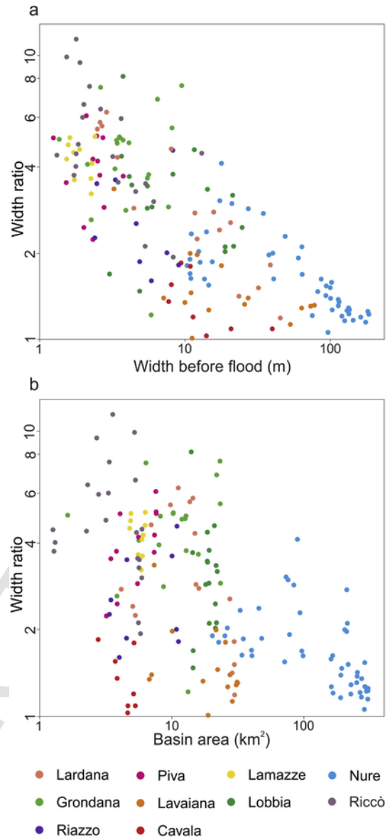
Fig. 5. Scatterplot of width ratio versus channel width before the flood event (a) and versus basin area (b).
