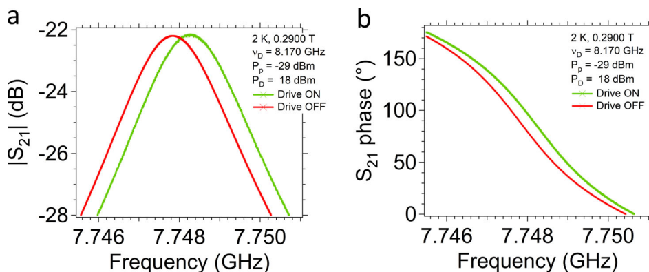
Figure 4. Dispersive shift of a) transmission and b) phase of the resonator measured for the DPNO spin ensemble at 2 K, B_0 = 0.2900 T, and for \theta = 90^\circ when the MW drive is turned ON (green trace) or kept OFF (red trace) at \nu_s = 8.1705 GHz. Probe and drive powers are P_{in,p} = -29 dBm and P_{in,D} = +18 dBm, respectively.
