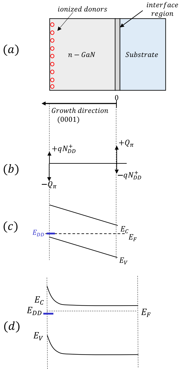
Figure 8: (a) schematic representation of a n-type GaN layer grown on a substrate. The (defective) interface region is shown. (b) charge diagram showing the screening induced by surface donors. (c) band diagram showing the surface donor level approaching the Fermi level at the surface of GaN, thus leading to the generation of the screening charge qN_{DD}^+ . (d) band diagram for a thick
