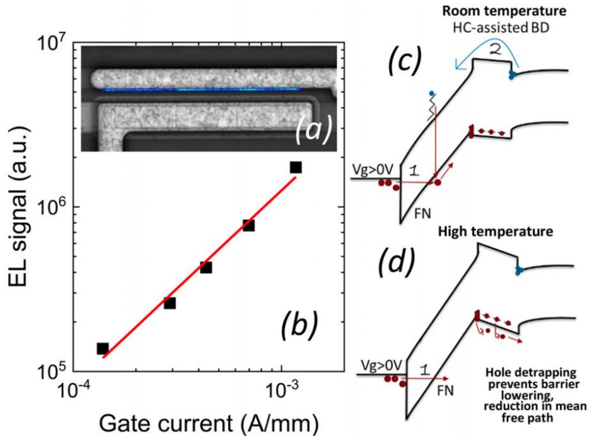
Figure 85: (a) spatial distribution of the electro-luminescence and (b) its correlation with the gate current. (c-d) sketch of the degradation process leading to a higher robustness at high temperature in p-GaN gate devices. Reprinted from F. Masin et al., "Positive temperature dependence of time-dependent breakdown of GaN-on-Si E-mode HEMTs under positive gate stress", Applied Physics Letters 115, 052103 (2019) https://doi.org/10.1063/1.5109301 , with the permission of AIP Publishing [586].
