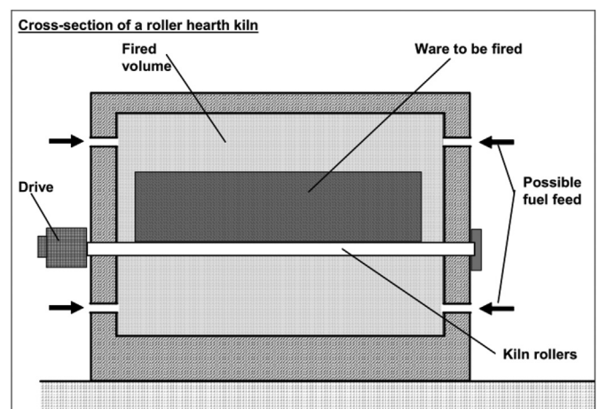
Fig. 2. Cross-section of a roller hearth kiln [3].
