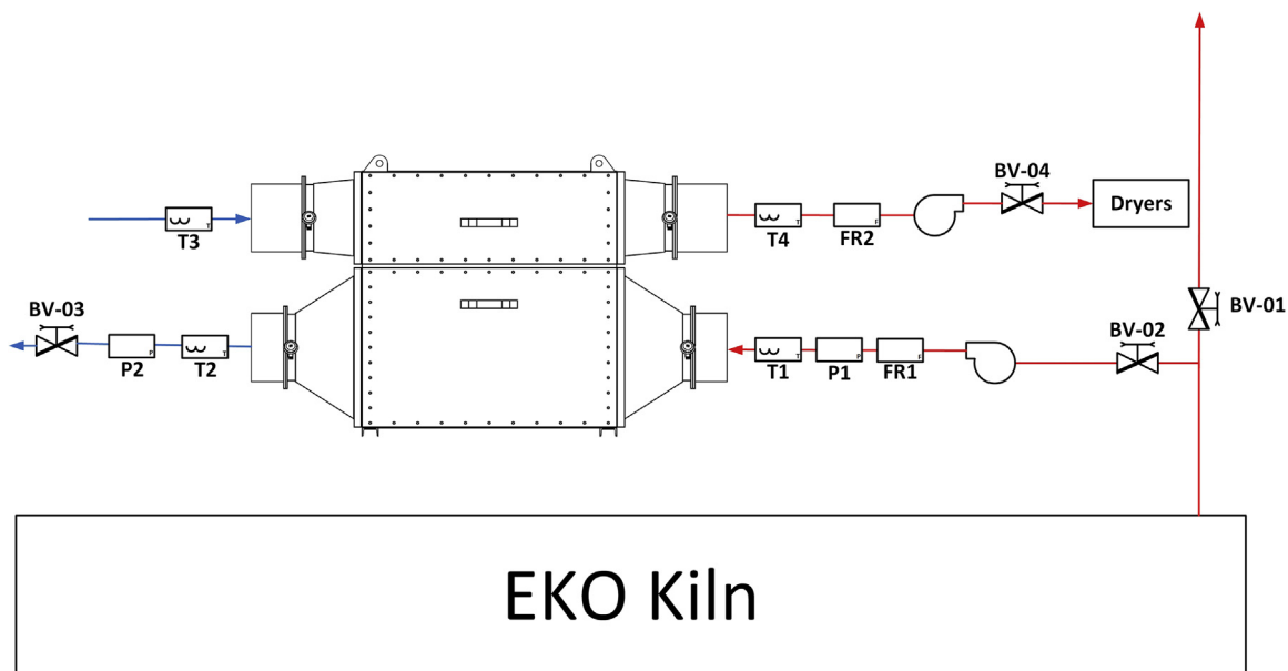
Fig. 6. HPHE P&ID system.
