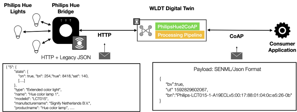
Fig. 5. Example of a WLDT instance mirroring Philips Hue lights through the standard use of CoAP and SenML.
