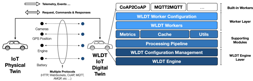
Fig. 1. Basic structure and main modules of White Label Digital Twin.
