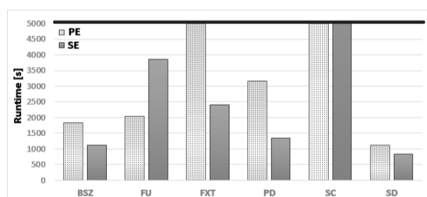
Fig. 5. Collapsing performance of different collapsing tools. Total computational time for collapsing SE and PE samples, respectively.
