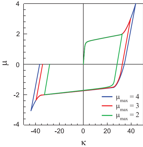
Figure 6. Normalized cyclic variations of the applied bending moment with the beam curvature, under alternative loadings for \mu_{\max} = 2, 3, \text{ and } 4 , for Brinson SMA material.
