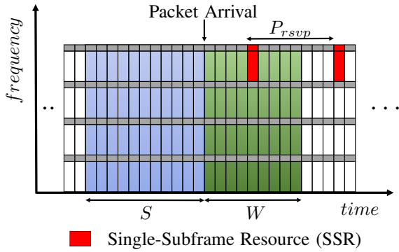
FIGURE 1. C-V2X Resource Grid Arrangement
