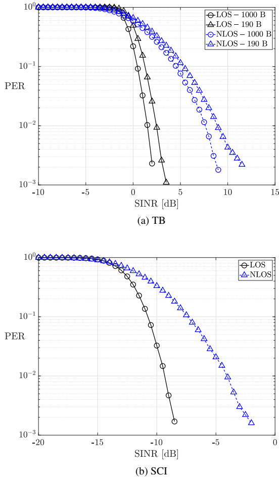
FIGURE 3. PER as a function of average SINR
