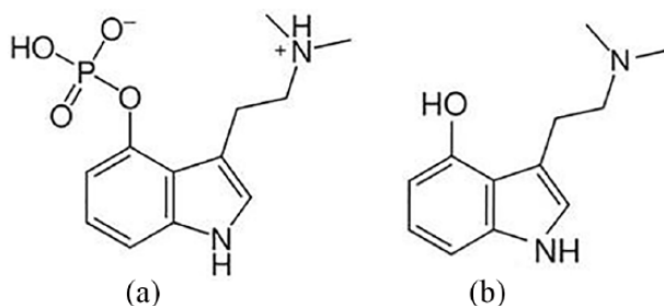
Figure 1. The structure of (a) psilocybin and (b) psilocin.
