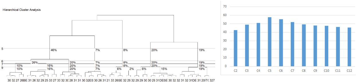
Figure 4 – Dendrogram and Calinski and Harabasz index
