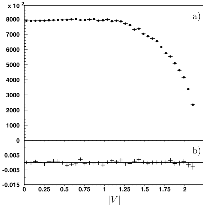
Fig. 3. a) Experimental |V| distribution obtained by projection of the (U, |V|) distribution used in the two-dimensional fit to extract the k parameter, after correction for the trigger inefficiency. b) Deviation from 1 of the ratio between the experimental and normalized simulated distributions for the best two-dimensional fit parameters.
