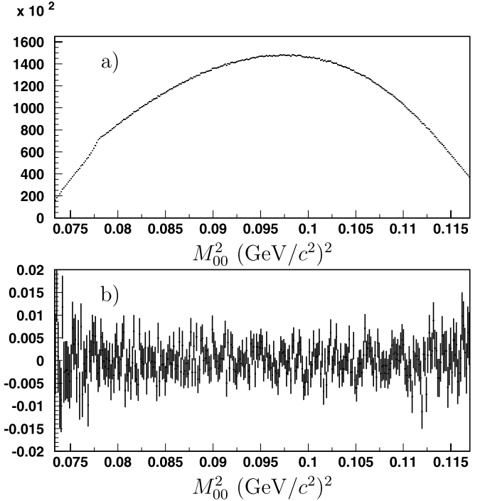
Fig. 2. a) Experimental distribution of the square of the \pi^0\pi^0 mass, M_{00}^2 , from K^\pm \rightarrow \pi^\pm\pi^0\pi^0 decay in the fit region. b) Relative deviation of the experimental spectrum from the best fit result (Data - Fit)/Fit .
