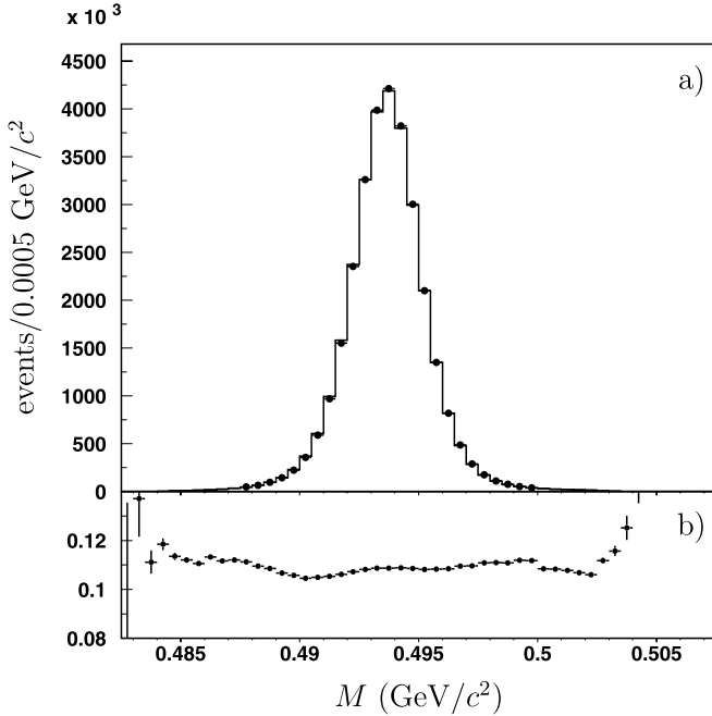
Fig. 1. Reconstructed \pi^\pm\pi^0\pi^0 invariant mass ( M ) distributions for data and MC simulation. a) Experimental (solid circles) and simulated (histogram) distributions, normalized to the number of data events. b) Ratio between the experimental and simulated distributions before this normalization.
