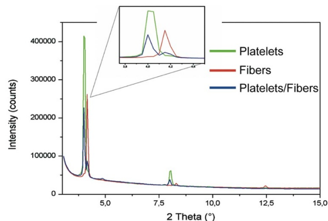
Figure 3 | X-Ray diffraction. Diffraction patterns of three different films on a Si/SiO 2 substrate having a majority of platelets (green curve), fibers (red curve) and a mixture of platelets and fibers (blue curve).
