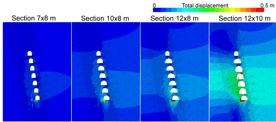
Figure 6: Stability analysis of Montevectchia mine: tunnel convergence of VS tunnel section.
