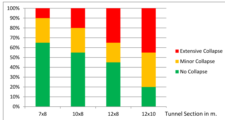
Figure 9: Summary graph of the 80 simulations performed to take into account the variability and uncertainty of input data at the Montevchia mine site.
