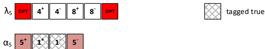
Figure 12: public and private trips at the end of createPrivateTrip()
