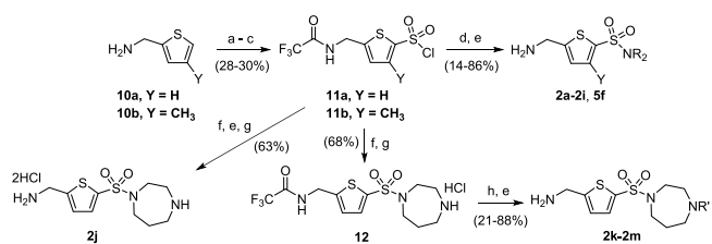
Scheme 1. General Synthetic Routes to AMT-Sulfonamide Analogues 2a–n and 5f a
