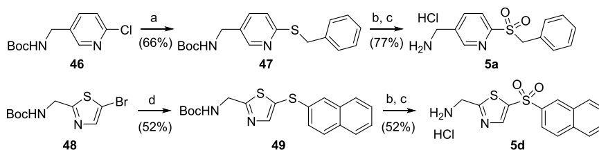
Scheme 13. Synthetic Routes to Aminomethylene-Pyridine, Aminomethylene-Thiazole, and Aminomethylene-Imidazole 5a and 5d a
