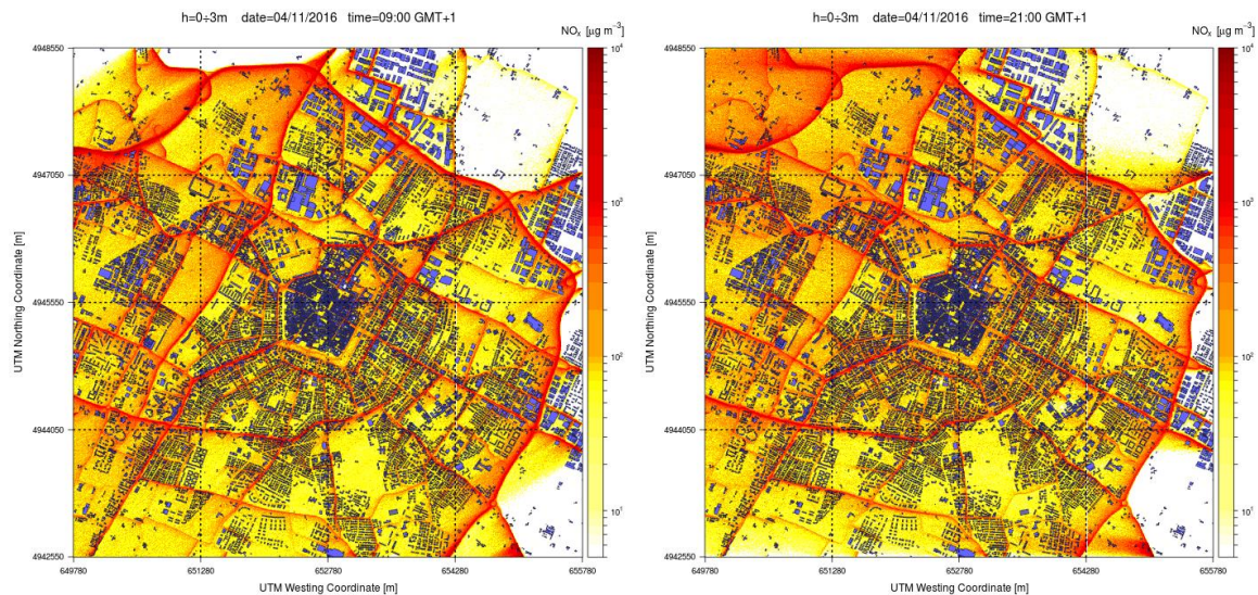
Figure 3. \text{NO}_x hourly concentrations maps on November 4 th 2016, from 8:00 a.m. to 9:00 a.m. on the left and from 8:00 p.m. to 9:00 p.m. on the right.
