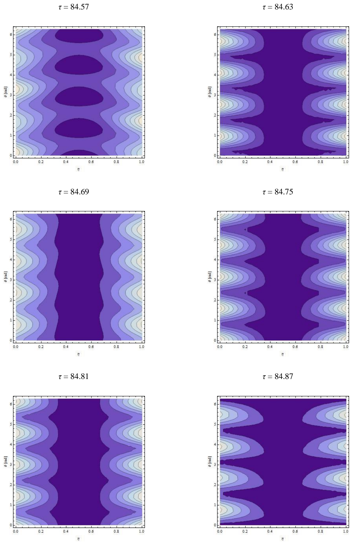
Figure 21. Contour plot of the total energy distribution \tilde{E}(\eta, \theta, \tau) of the conjugate modes (1,2), (1,2,c) over the SWCNT surface (\eta, \theta) . Backward travelling wave from \theta = 2\pi to \theta = 0 in the time range \tau = (84.57, 84.87) .
