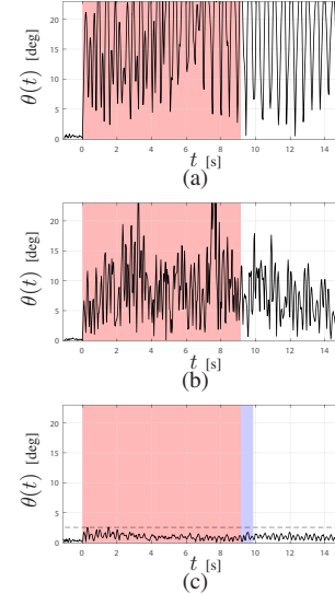
Fig. 10. Sloshing angle profiles measured when the liquid vessel is moved according to the trajectories of Fig. 9: unfiltered trajectory (a); unfiltered trajectory with orientation compensation (b); smoothed trajectory with orientation compensation (c). The red area indicates the motion time while the blue area highlights the time lag T introduced by the filter.
