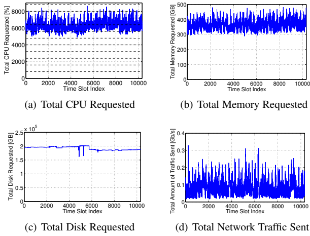
Fig. 2. Evolution of the CPU, memory, disk and network traffic vs TS index for the considered DC trace.
