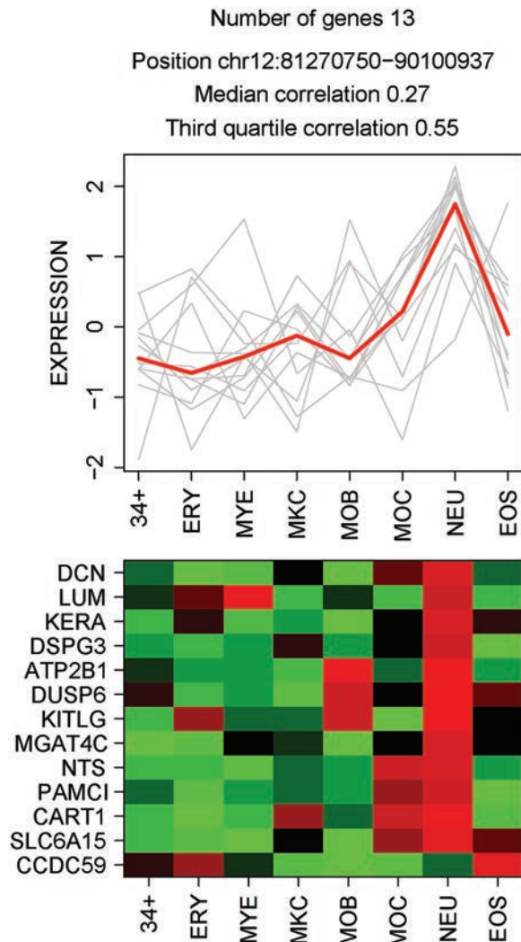
Figure 5. Example of a co-expressed region. Expression plot and heat-map, with genes ordered by genomic position, describing a region of chromosome 12 (81 270 750 – 90 100 937) harbouring 13 co-expressed genes. The red-bold line represents the median of expression profiles in the gene set. (34+: CD34+HSC; ERY: Erythroblasts; MYE: Myeloblasts; MKC: Megakaryoblasts; MOB: Monoblasts; MOC: Monocytes; NEU: Neutrophils; EOS: Eosinophils).
