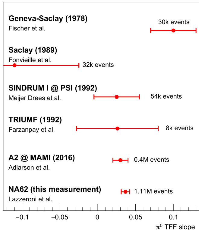
Fig. 4. Comparison of the \pi^0 TFF slope measurements in the time-like momentum transfer region [11–15].
