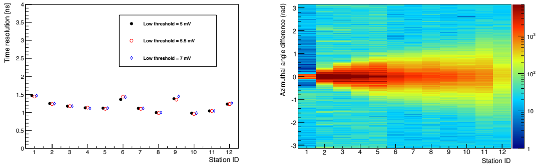
Figure 37. Left: time resolution for LAV stations for a high threshold of 15 mV and three different values of the low threshold. Right: difference in azimuthal angle between a cluster reconstructed in the most upstream layer of LAV station 1 (ID = 1) and clusters in successive layers, as a function of station ID, for data from a muon run.
