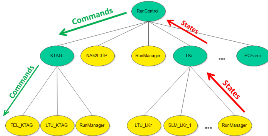
Figure 70. Tree-like hierarchy of units. Green shapes are logical units and yellow shapes are device units. Commands are propagated downwards and states are propagated upwards and summarized in the logical units.
