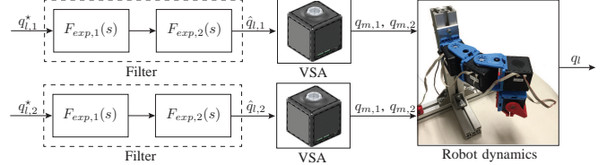
Fig. 9. Block-scheme representation of the feedforward control.
