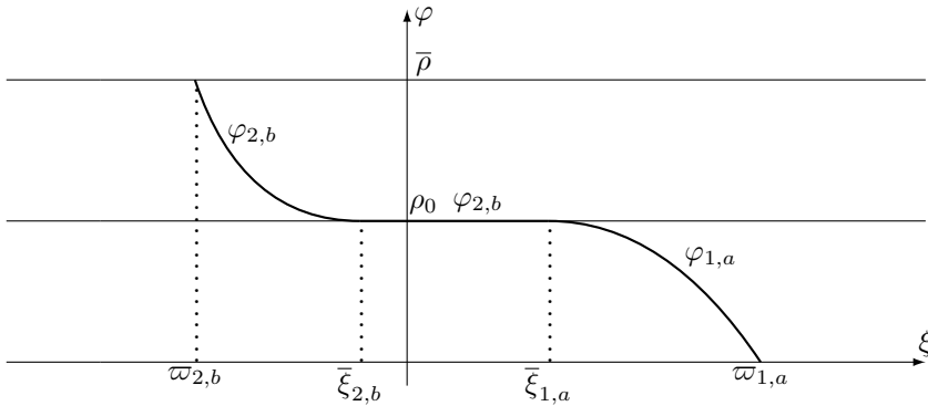
FIGURE 9. The profile \bar{\varphi}_1 in (7.5).
