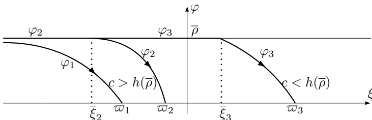
FIGURE 3. A strictly decreasing classical profile \varphi_1 occurring in case (i); a non-strictly decreasing classical profile \varphi_2 occurring in case (ii); a sharp profile \varphi_3 .
