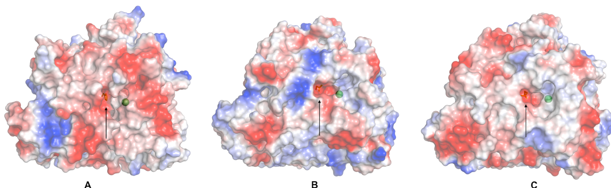
Figure 7. Surface charge distribution of McoG (A), Ta L (B) and Ma L (C); blue, positively charged regions; red, negatively charged regions. His253, Asp236 and Glu235 of these laccases, respectively, are indicated with an arrow.
