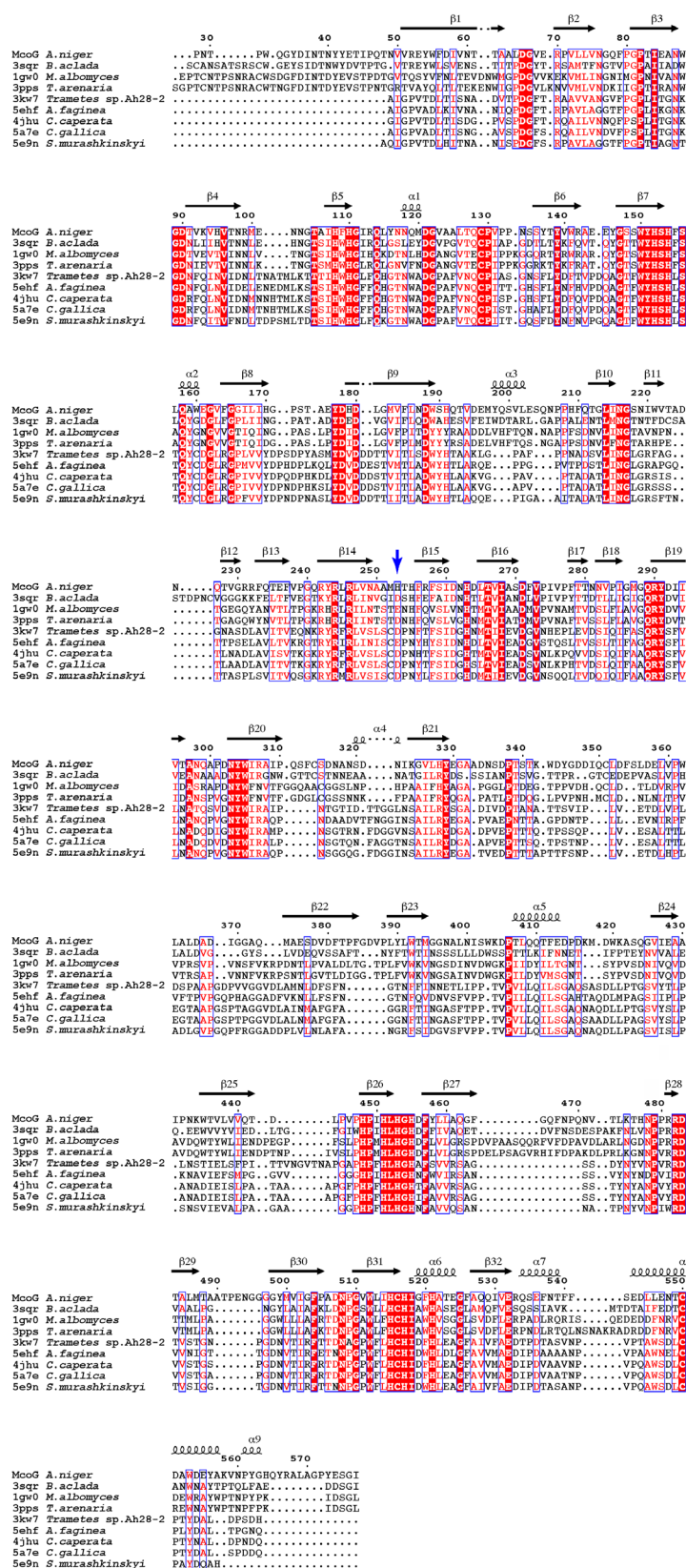
Figure 1. Alignment of the amino acid sequences for McoG from Aspergillus niger (5LM8) and for the laccases from Botrytis aclada (3SQR), Melanocarpus albomyces (MaL, 1GW0), Thielavia arenaria (TaL, 3PPS), Trametes sp. AH28-2 (3KW7), Antrodia faginea (5EHF), Corioloropsis caperata (4JHU), Corioloropsis gallica (5A7E) and Steccherinum murashkinskyi (5E9N). Completely conserved residues are shaded with a red background. The position of residue 253 ( A. niger McoG numbering) is indicated with a blue arrow.
