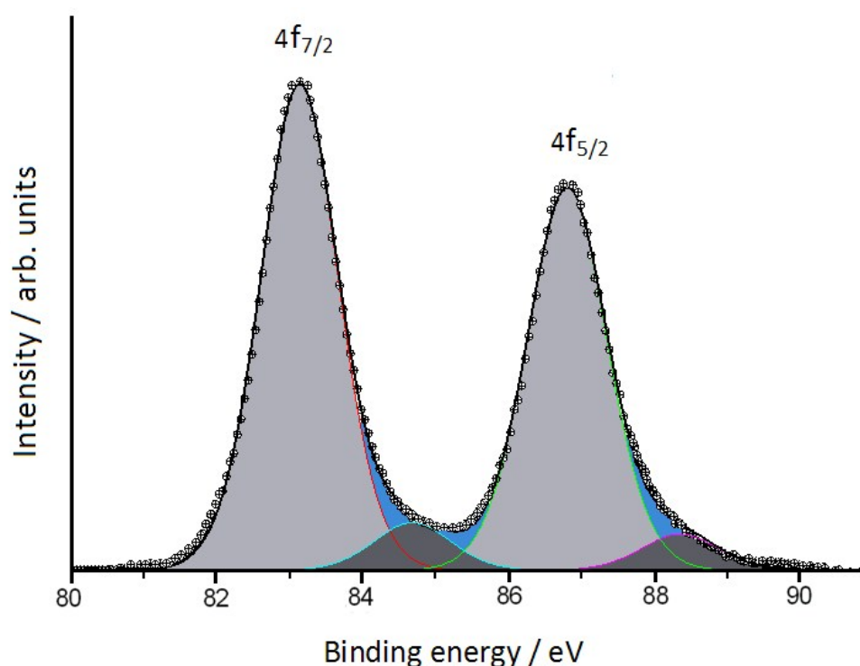
Fig. 5 – Deconvolved XPS spectrum of deposited Au nanoparticles (4f 7/2 and 4f 5/2 transitions). Circles represent experimental points, while light gray and dark gray the contributions of Au(0) and Au(I), respectively.
