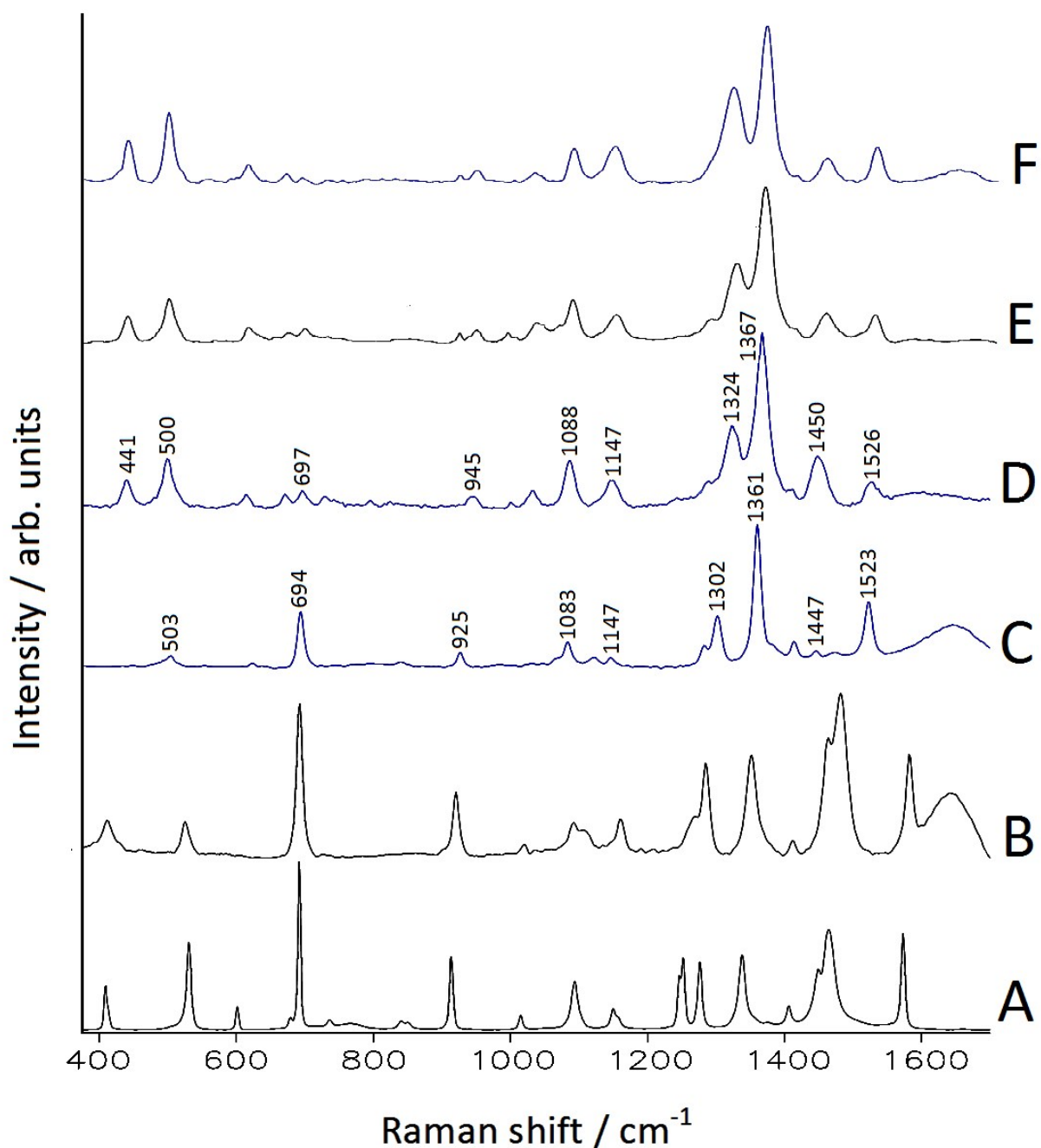
Fig. 2 – Raman spectra of TZ as solid sample (A), in neutral (B) and alkaline (C) solution ( 10^{-1}\text{M} concentration). The SERS spectra of TZ in Au colloid ( 10^{-5}\text{ M} concentration) obtained by different laser excitations (D: 647.1 nm; E: 785 nm; F: 1064 nm) are reported for comparison.
