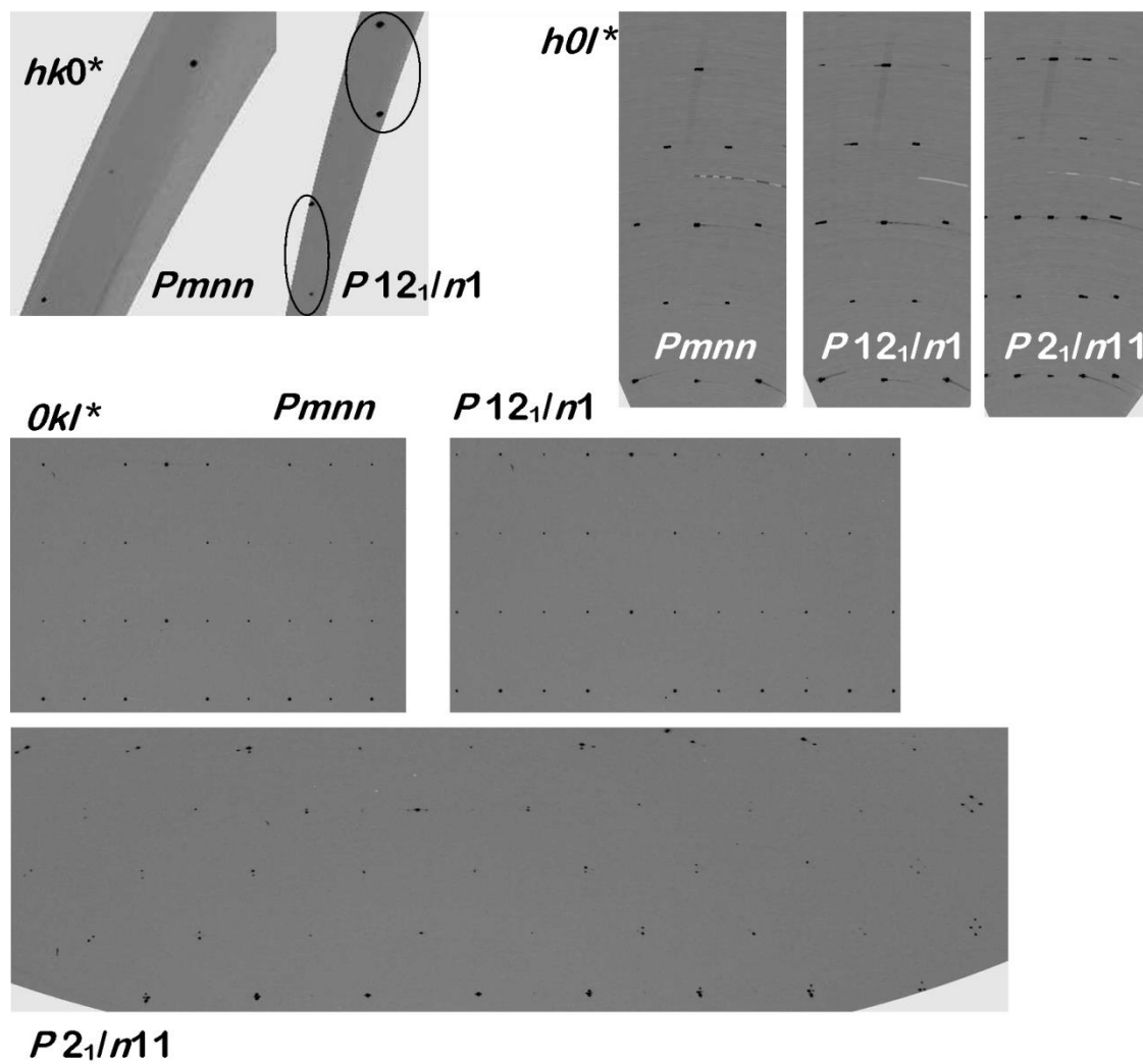
Figure 4. Reconstruction of selected reciprocal lattice planes of the Pmnn -, P12_1/n1 - and P2_1/n1 -polymorphs of Si-FER, based on the single-crystal experiment using silicone oil as P -transmitting fluid.
