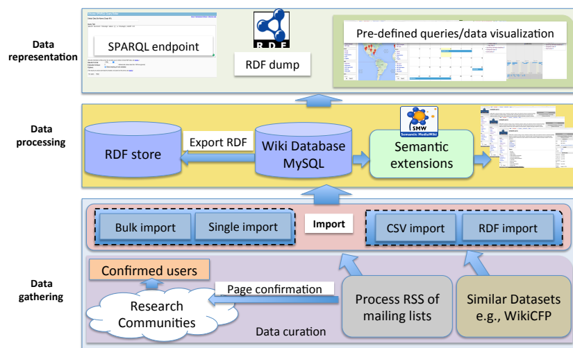
Figure 2: OpenResearch Architecture
