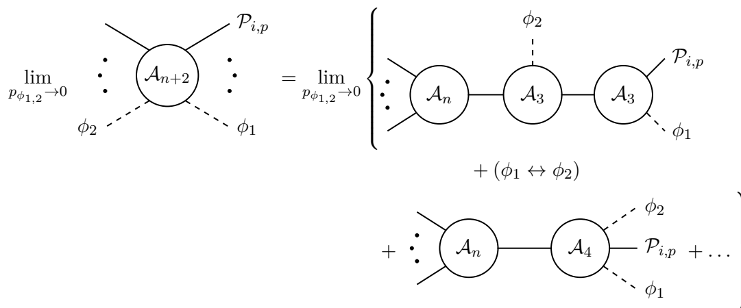
Figure 2. Schematic diagrammatic representation of eq. (2.23) for an amplitude with two ALPs ( m = 2 ). The first line represents the insertion of two 3-point amplitudes, the second one is the Bose exchange of the two ALPs in the double \mathcal{A}_3 insertion, while the last line represents the insertion of the 4-point amplitude with two ALPs whose coefficients need to be determined. The dots denote other factorization channels that are automatically regular in the double soft limit.
