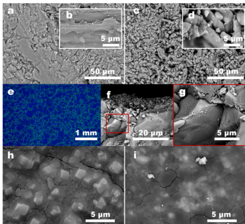
Fig. 2. Surfaces of freshly quarried a-b) Apuan Marble and c-d) Lumaquela de Ajarte displaying differing roughness as observed with a secondary electron detector. e) Inter- and intra-granular microcracks in the fabric of Apuan Marble after thermal treatment. The visualization of cracks was performed using UV-light on a thin section embedded in a fluorescence resin. f-g) SEM images of a broken fragment of a thermally treated Apuan Marble sample showing f) precipitates on the surface, and g) a honeycomb-like texture, possibly as a result of beginning thermal degradation, located at an intergranular boundary in the vicinity of the surface. h) Backscatter electron images of embedded rhombohedral crystal in the nanosilica matrix on the surface of thermally treated Apuan Marble and, i) secondary electron images of the discoloration of the nanosilica matrix due to calcium mobilization on surfaces of thermally treated Lumaquela de Ajarte.
