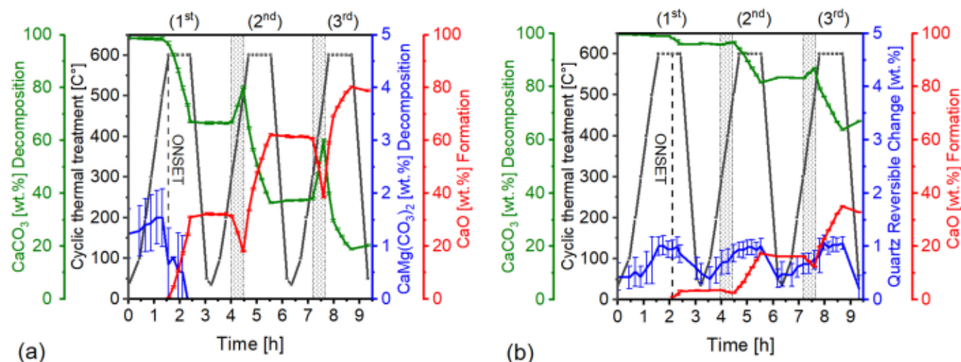
Fig. 3. Phase evolution (wt%) with temperature obtained from Rietveld refinement of in-situ XRD patterns for a) Apuan Marble and b) Lumaquela de Ajarte. Shaded areas highlight the retrograde reaction (in the second and third heating ramp) while the dotted line indicates the onset of thermal decomposition during the isothermal treatment (only reported for the first thermal cycle). (For interpretation of the references to colour in this figure legend, the reader is referred to the web version of this article.)
