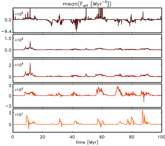
Figure 3. Eulerian analysis: evolution of the mean values of effective dynamical term. The mean values are computed within pairs of short cylinders aligned with the bipolar jet path, with a cylindrical radius of 15 kpc and increasing distance from the AGN ( \approx 1, 9, 18, 36, 72 kpc; dark red to bright yellow colour/top to bottom panel). This plot is the replacement for the second panel of fig. 4 in the original paper. However, due to the large spread in amplitudes, we do show the results for each cylinder separately and not in the same plot. The evolution of the mean effective source term is significantly different to the one in the original paper. This is inherent to the baroclinic term, which can locally dominate the mean.
