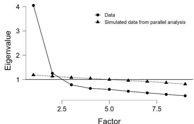
Fig. 1. Scree plot.
