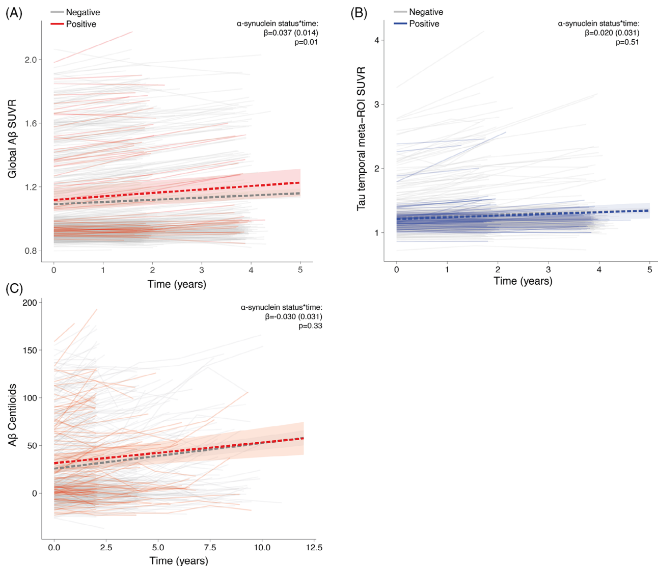
FIGURE 3 Effect of \alpha -synuclein status on longitudinal A\beta - and tau PET. Linear mixed effect models investigating the effect of \alpha -synuclein status on longitudinal global neocortical A\beta SUVR ( n = 567 ) (A) and temporal tau PET SUVR ( n = 596 ) (B) in BioFINDER-2, and A\beta Centiloids in ADNI ( n = 473 ) (C). Linear mixed effect models with random slope and intercept were fitted, including age and sex as covariates. Standardized beta coefficient (standard error) and p value of \alpha -synuclein status \times time is reported on each graph. Negative/positive indicates CSF \alpha -synuclein status. \alpha -synuclein, alpha synuclein; A\beta , amyloid beta; AD, Alzheimer's disease; ADNI, Alzheimer's Disease Neuroimaging Initiative; BioFINDER-2, Biomarkers for Identifying Neurodegenerative Disorders Early and Reliably Two; CSF, cerebrospinal fluid; PET, positron emission tomography; SUVR, standardized uptake value ratio.
