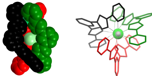
Fig. 3 (Left) Space-filling representation of the supramolecular cation (\text{Cl}@\text{[Ni}_2\text{L}_3\text{]})^{3+} of compound 1 , with ligands shown in red, green and black, respectively. (Right) View of the species (\text{Cl}@\text{[Ni}_2\text{L}_3\text{]})^{3+} along the Ni...Ni axis, emphasizing the helical arrangement engendered by the ligand twisting around the C–C bonds that connect the central m -phenylene unit to the pyrazolylpyridine groups.
