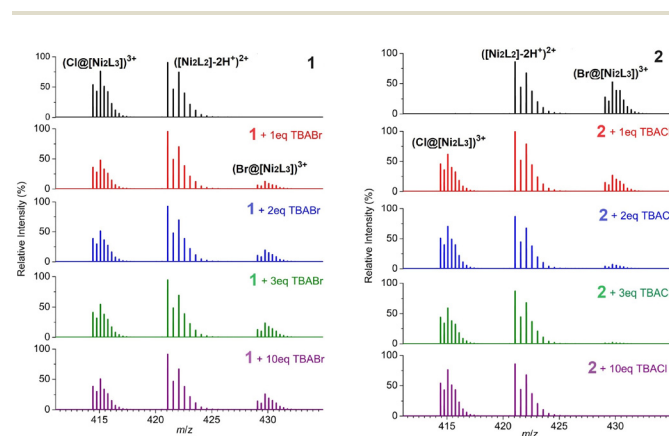
Fig. 4 Selected region ( m/z = 411 to 435) of the ESI-MS spectrogram of compounds 1 (left) before and after the addition of different amounts of TBABr and TBACl, respectively (direct infusion, MeCN, positive ion mode).
