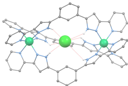
Fig. 2 Representation of the supramolecular cation (\text{Cl}@\text{[Ni}_2\text{L}_3\text{]})^{3+} of compound 1 . The large green ball is Cl, medium green balls are Ni, blue balls are N, grey balls are C and white balls are H. Only H atoms from N–H groups are shown. H-bonds are dashed red lines.
