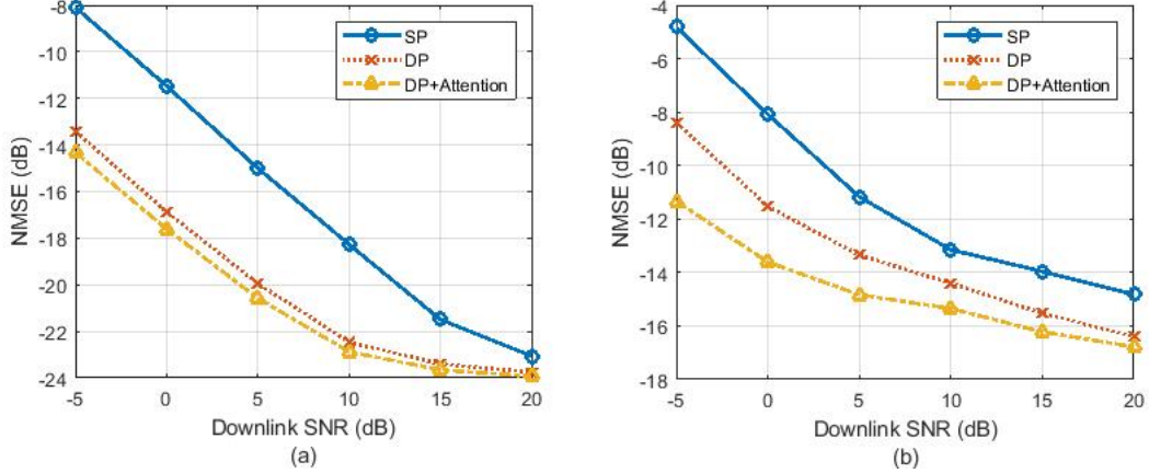
Fig. 7: Comparison between the NMSE (dB) values achieved using same pilots (SP) over all subcarriers [10] and the proposed frequency-aware pilot design scheme (DP) for N = 32, M = 256 , (a) L = 16 , (b) L = 12 .
