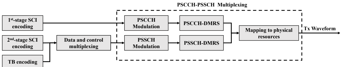
Fig. 2. Transmitter chain.
