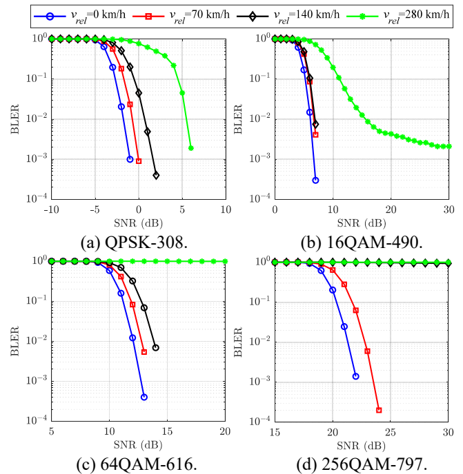
Fig. 5. Impact of the Tx-Rx relative speed on the TB BLER for different TB MCSs.
