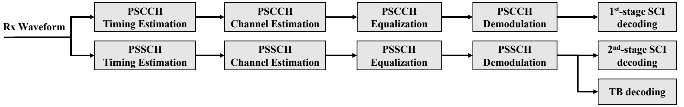
Fig. 3. Receiver chain.
