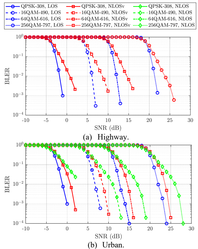
Fig. 7. TB BLER as a function of the SNR for different channel models and states.
