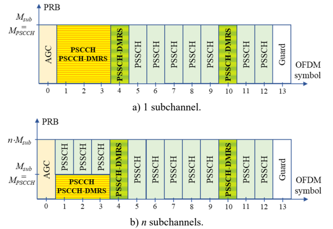
Fig. 1. PSCCH and PSSCH multiplexing in NR V2X SL: normal cyclic prefix, 3 PSCCH OFDM symbols and 2 PSSCH-DMRS symbols.
