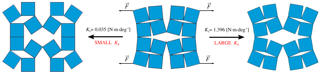
Figure 3. Diagrams showing the final state of the deformation of two systems, where the hinging process is governed by friction, with K_h values of 0.035 \text{ N} \cdot \text{m} \cdot \text{deg}^{-1} and 1.396 \text{ N} \cdot \text{m} \cdot \text{deg}^{-1} . Animations presenting the entire deformation range of these systems are provided in the Supplementary Information: ANIM1.gif and ANIM2.gif respectively.
