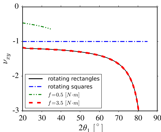
Figure 4. A plot showing a comparison of the Poisson's ratios obtained from the numerical solutions presented here for f = 0.5 \text{ N} \cdot \text{m} and f = 3.5 \text{ N} \cdot \text{m} with those calculated from analytical models for uni-level rotating rigid rectangle and square systems.
