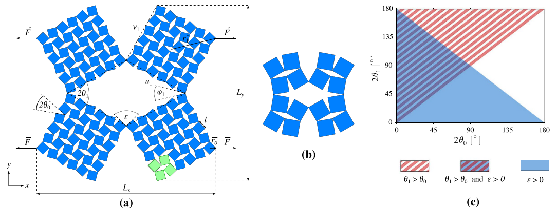
Figure 1. The panels in this figure present (a) the two-level hierarchical auxetic system with four square-like units corresponding to Level 1 of the structure, where each unit consists of N_0 \times N_0 (in the provided example N_0 = 3 ) Level 0 repeat units (bright green), (b) an example of the structure corresponding to N_0 = 1 and (c) the permissible angles for \theta_0 and \theta_1 , which conditions ensure that the squares do not overlap with each other and the system retains the same connectivity. This is attained when conditions \theta_1 > \theta_0 and \varepsilon = \pi - 2\theta_1 - 2\theta_0 > 0 are satisfied.
