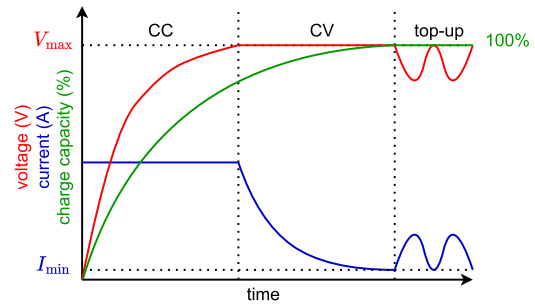
FIGURE 2. Typical charging curve of CC-CV protocol.
